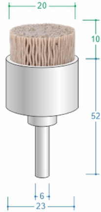
EB S6D20T10 RMP max 4500
