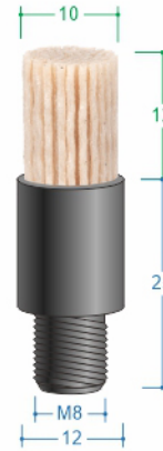
EB M8D10T12 RMP max 6000
