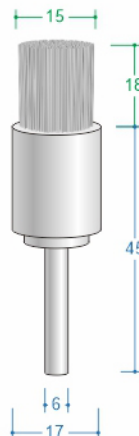
EB S6D15T18 RMP max 4500
