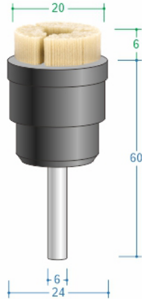
EB S6D20T6F3 RMP max 4500
