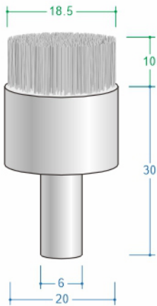
EB S6D18.5T10 RMP max 4500
