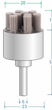
EB S6D20T10Z9 RMP max 4500
