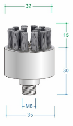
EB M8D32T15Z16 RMP max 4500
