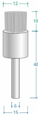
EB S6D12T10 RMP max 4500
