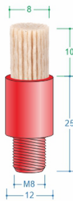
EB M8D8T10 RMP max 6000
