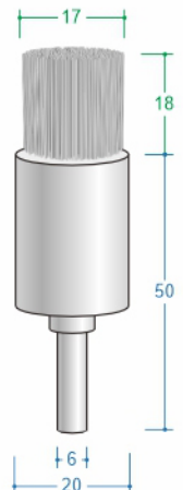
EB S6D17T18 RMP max 4500
