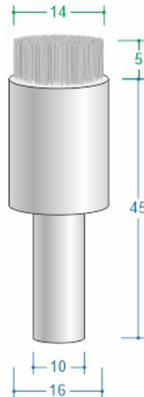
EB S10D14T5 RMP max 4500
