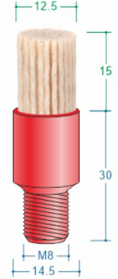
EB M8D12.5T15 RMP max 6000
